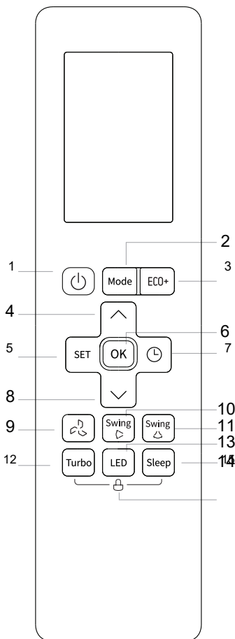
Model: RG10D4(F2S,G2S,H2S)/BGEF
